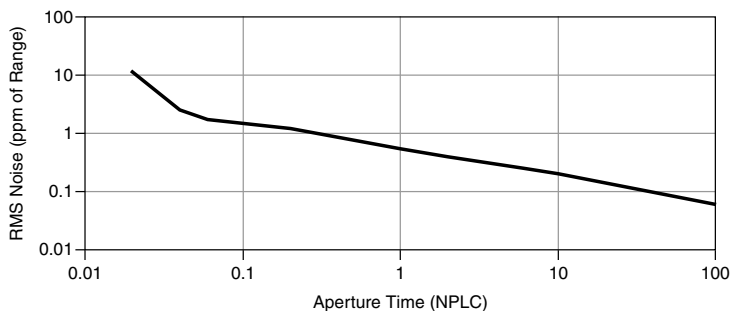
Figure 1. Noise Performance 2
